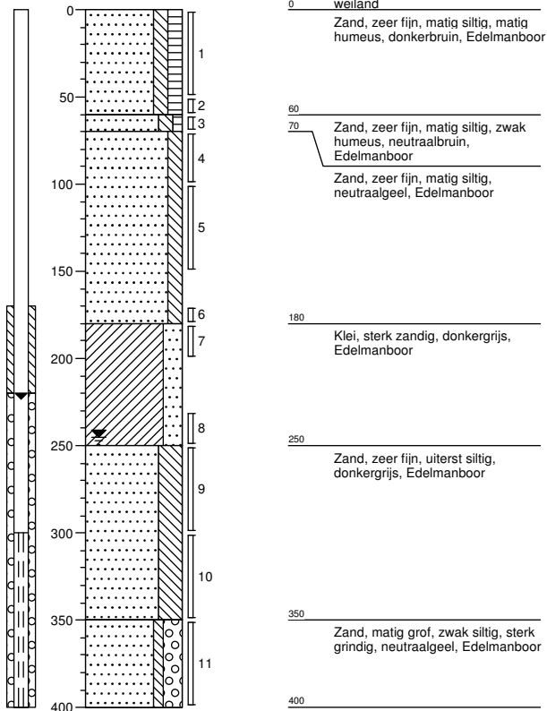
Boring: 01
